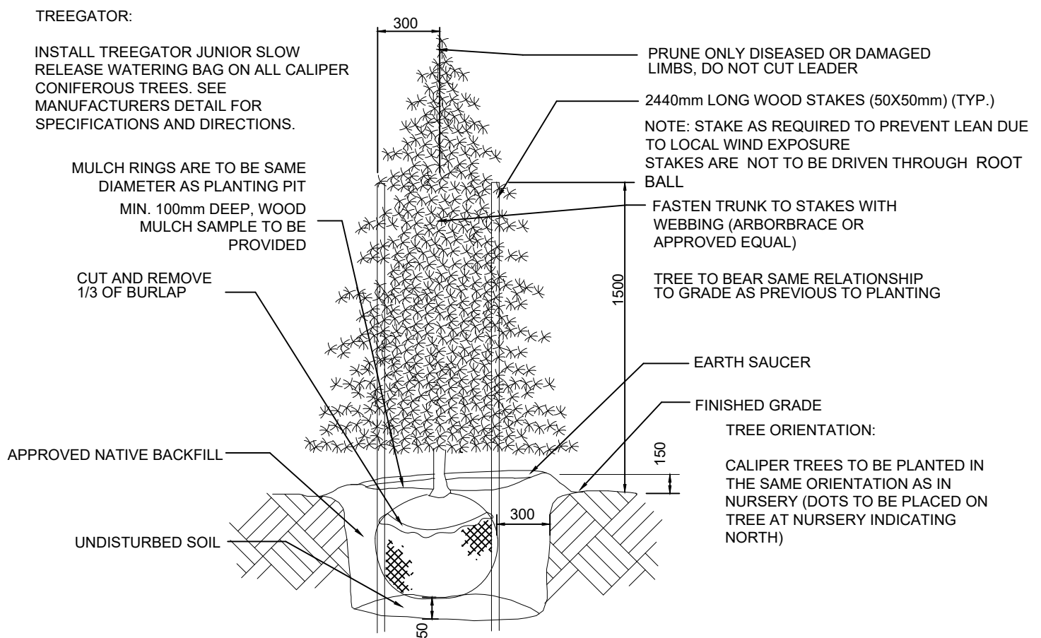
1 CONIFEROUS TREE PLANTING DETAIL NTS
